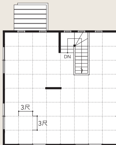
Base plan
